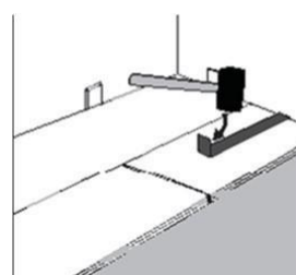
Step 8: Use hammer and pull bar to engage final piece, insert spacers and continue to next row.
