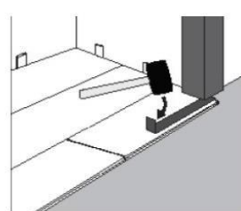
Step 7: Tap end of planks with hammer and tapping block to engage ends.
